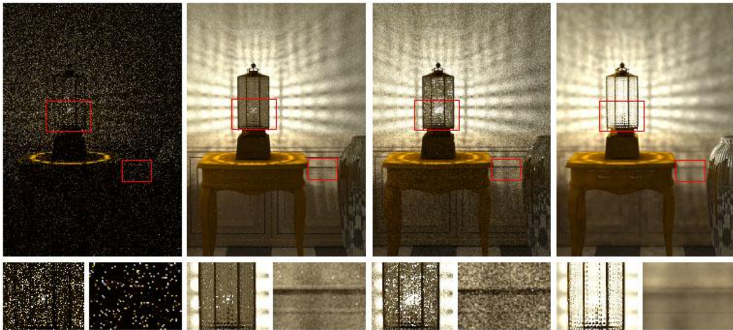
Path tracing
