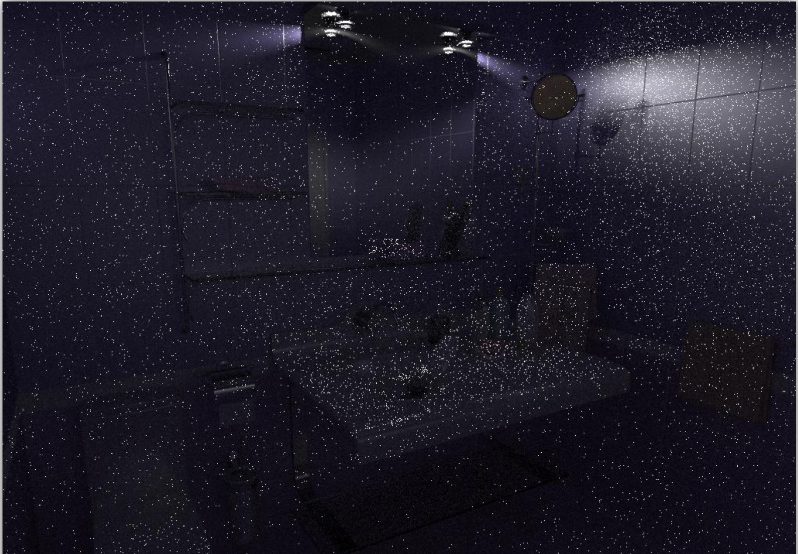
Path Tracing
